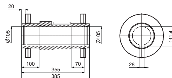
Hohlwelle / hollow shaft (SK5x07 / SK6x07)
