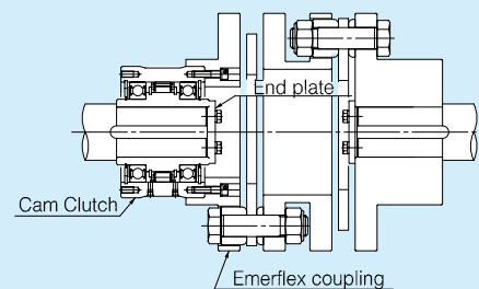
Installation example 3:
