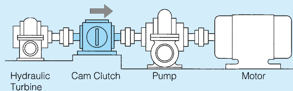
Example of energy saving pump (power recovery system)
