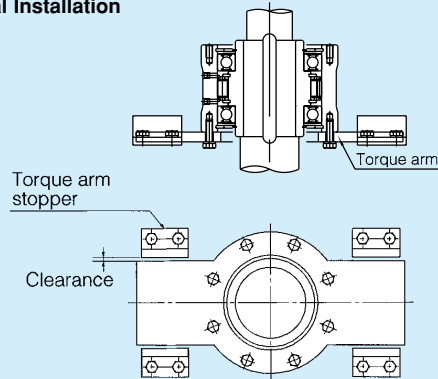
Installation example 2:
