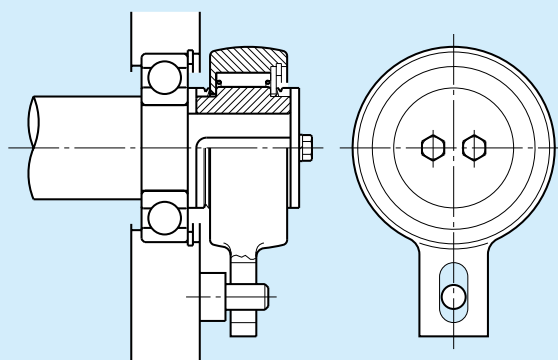
Typical Installation 2
