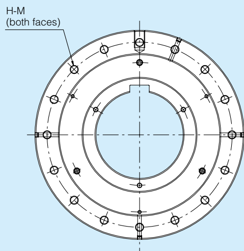
Chamfer of the bore end faces
