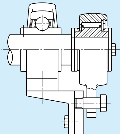
Typical Installation 1
