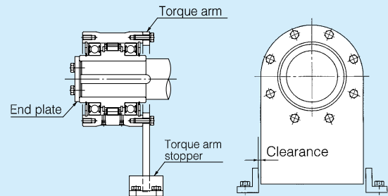
Installation example 1:
