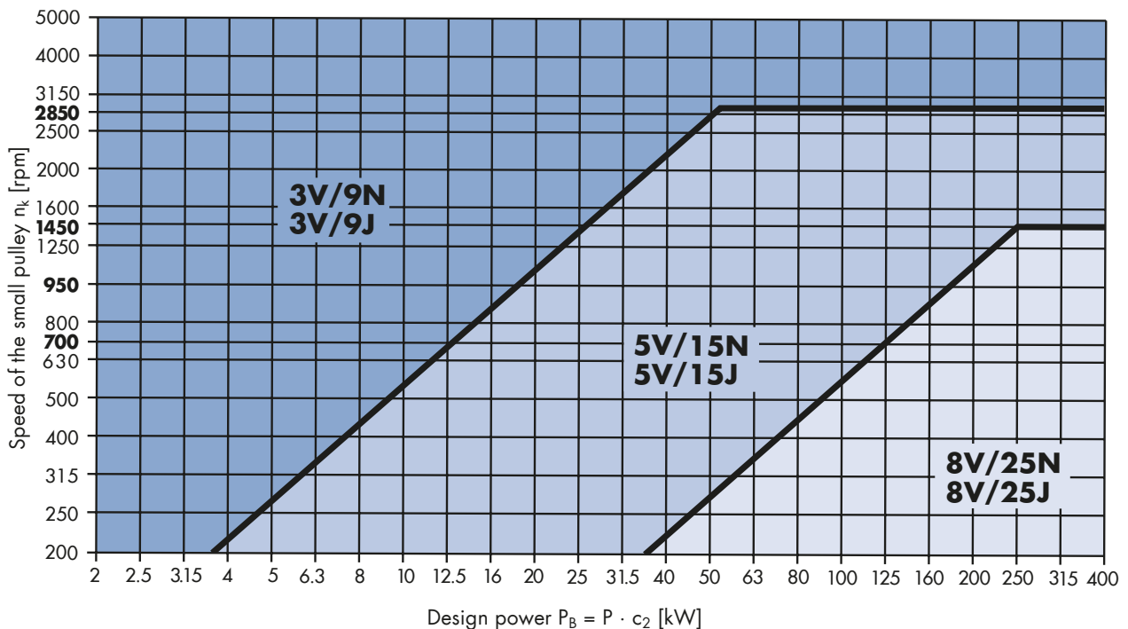
Diagram 3: optibelt SK high performance wedge belts ARPM/MPTA
