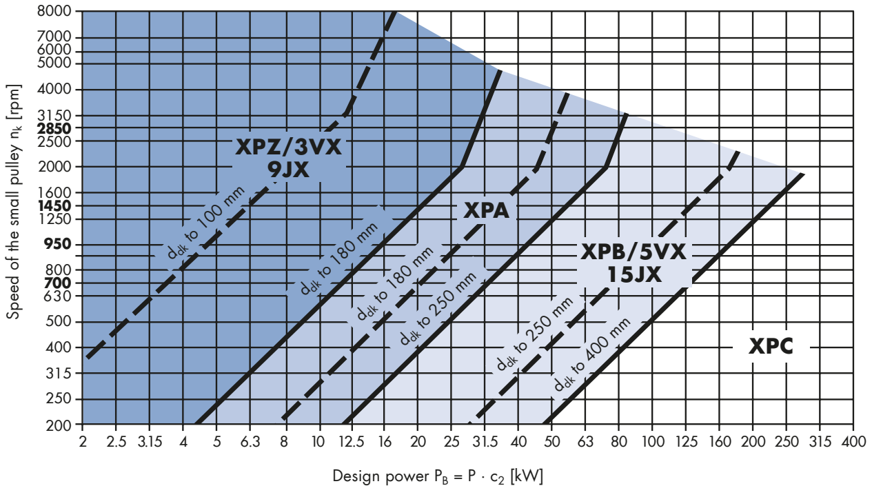
Diagram 4: optibelt SUPER X-POWER M=S wedge belts
