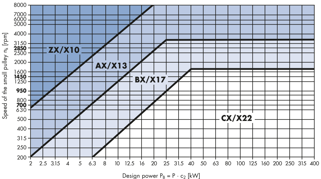
Diagram 5: optibelt SUPER TX M=S V-belts
