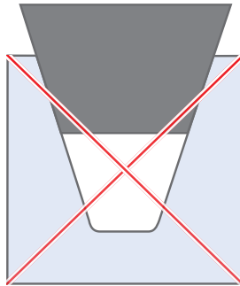
Belt too large / pulley groove too small
