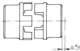
Axial misalignment
