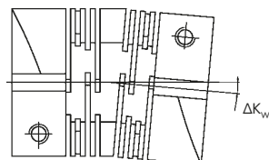
Angular misalignment
