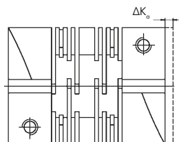
Axial misalignment
