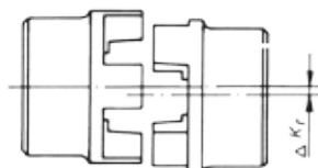
Radial misalignment
