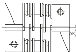
Radial misalignment
