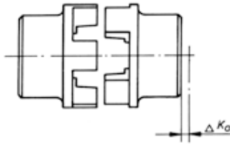
Axial misalignment
