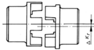
Radial misalignment
